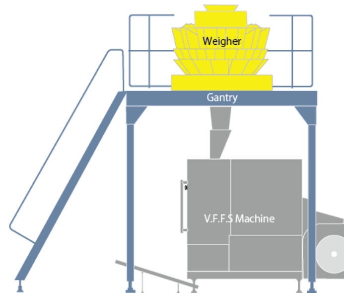
Multi-head weigher with gantry
